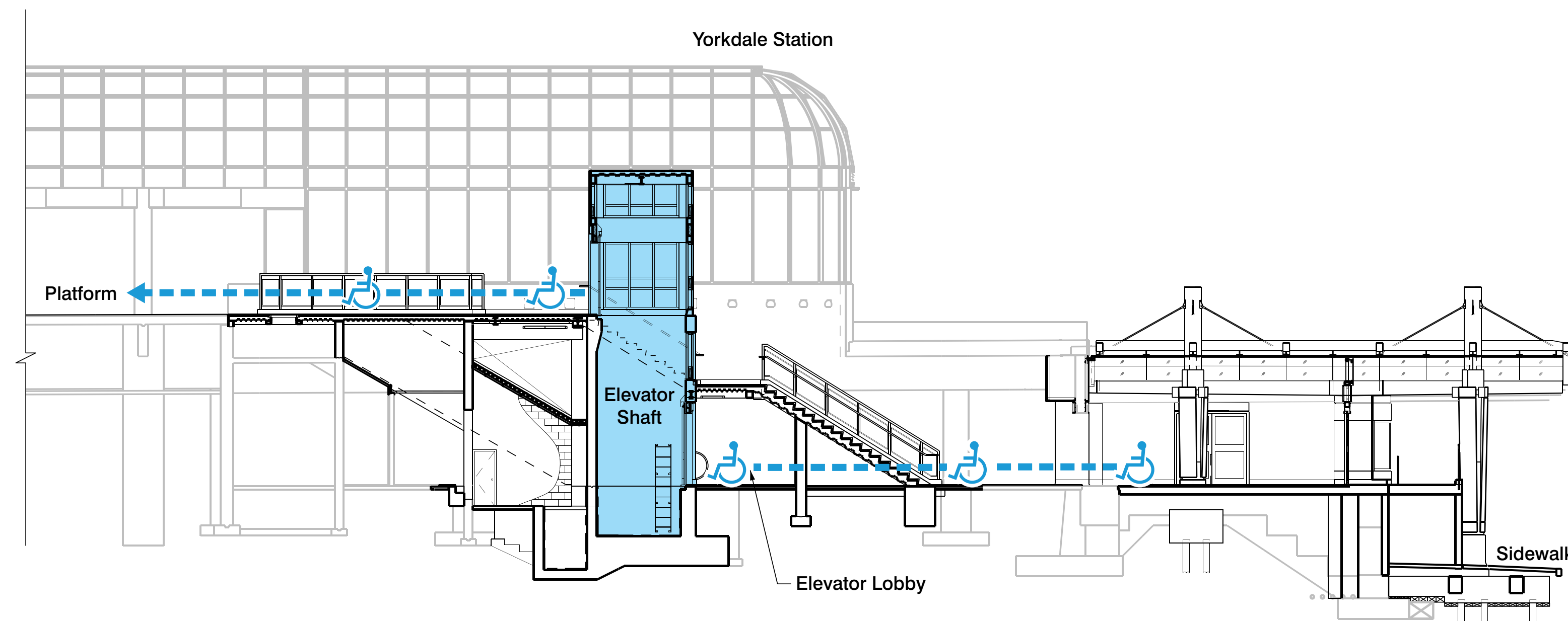
Cross Section
