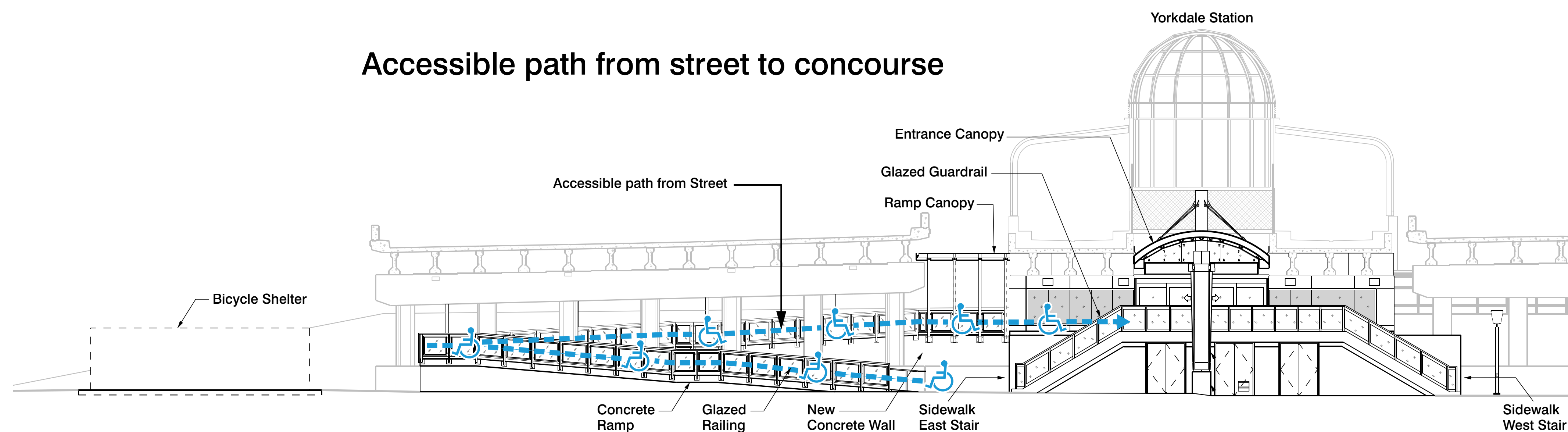
North Elevation
